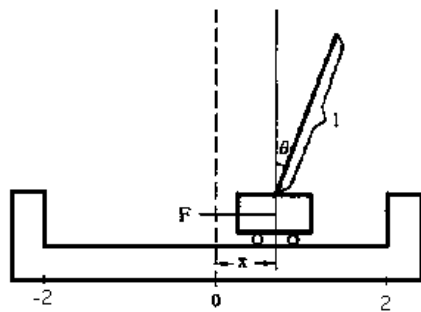
Figure 5. The cart-pole system
